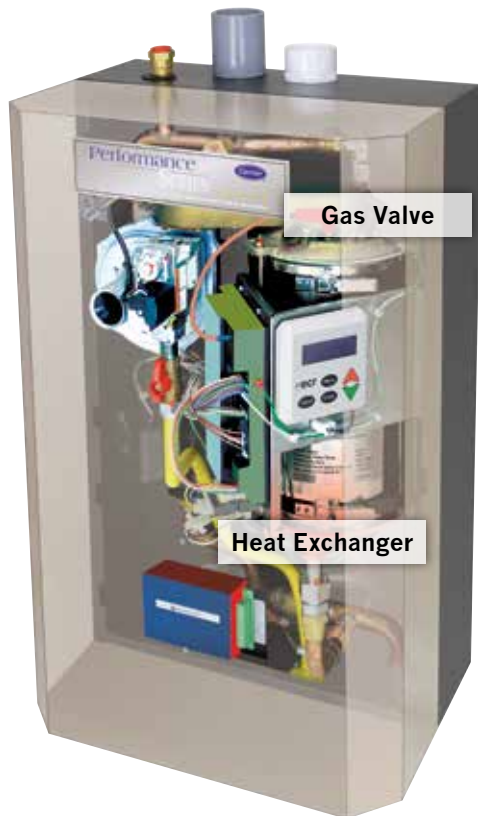
Performance™ 96 Model BWM Boiler shown
