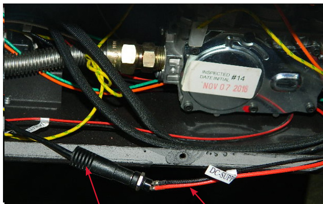
DC supply wire from wiring harness
