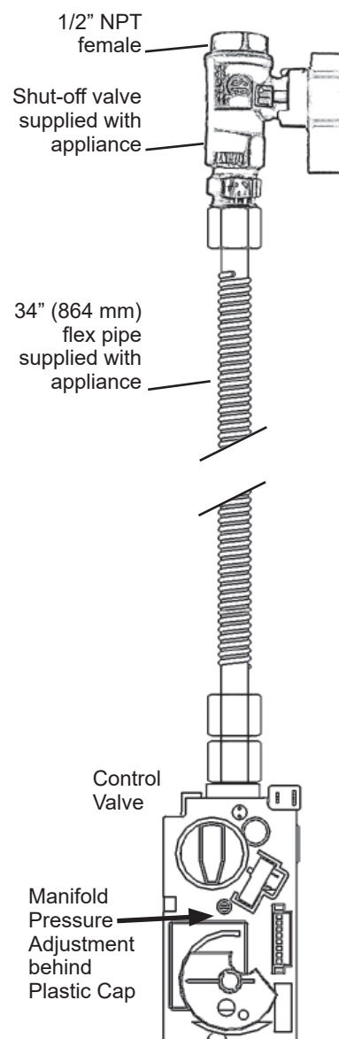
Valve Assembly
