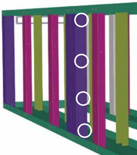
Diagram 10- Secure sections together with 4 screws through both inner corner Part Bs
