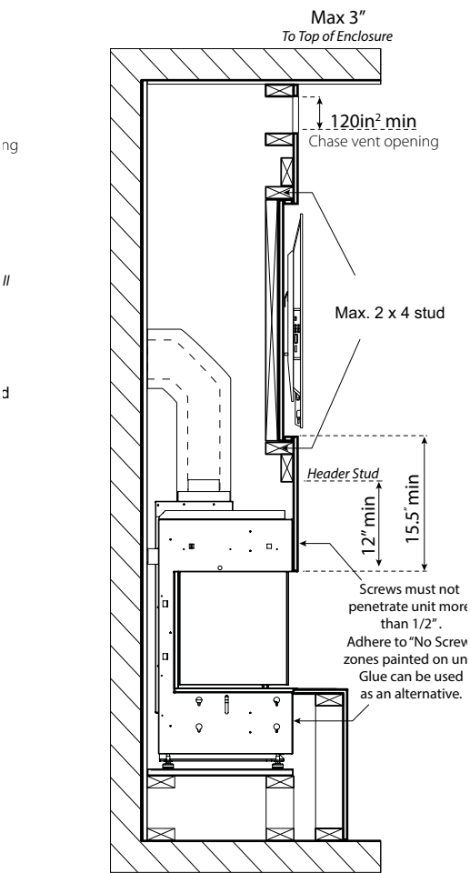
Flush wall TV recess using 1/2" drywall CB40E shown
