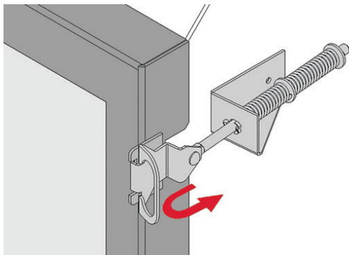
Spring-loaded window lever
