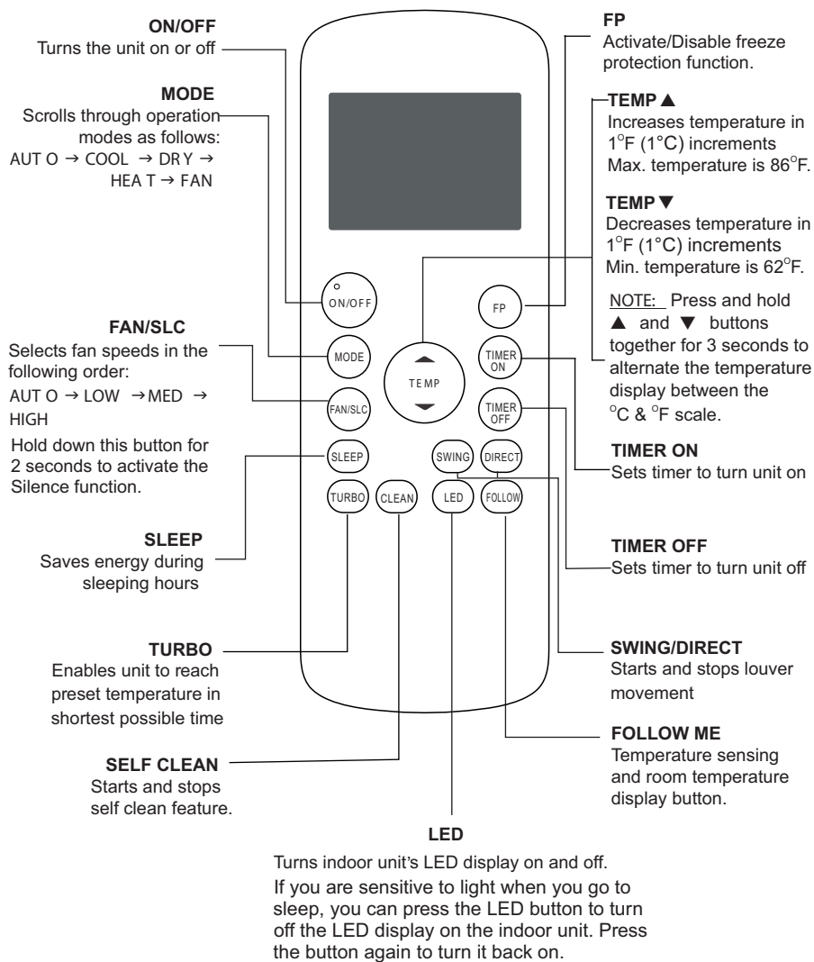
Fig. 2 Remote Controller
