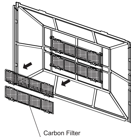
Fig. 17 – Carbon Filter
