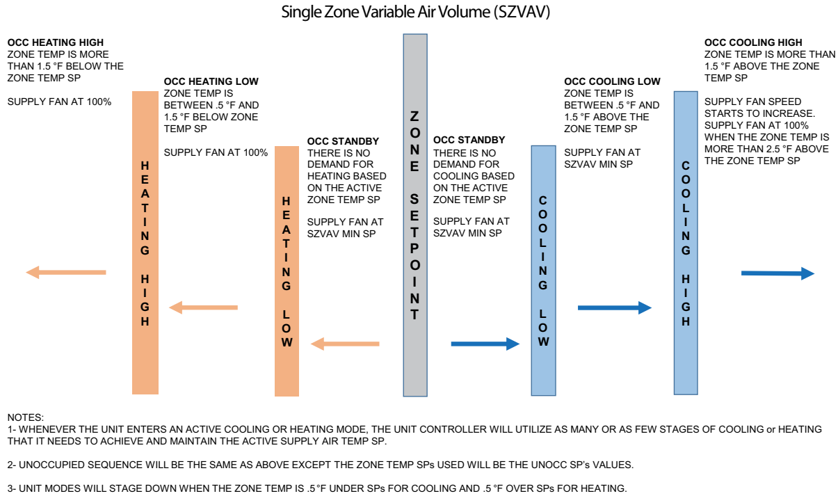
FIGURE 8 - OPERATIONAL MODE: SINGLE ZONE VAV
