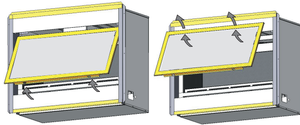
Figure 23g. Removing and installing the glass doors. Both sides typical.
