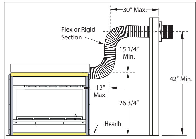
Figure 13b. Side Vented, wall mounted Multi-elbow termination installation. Installation for L38DF*-ST must have a minimum vertical rise of 42". The vent run must comply with the Venting Graph for Rear vent, wall mounted terminations, Figure 13.
