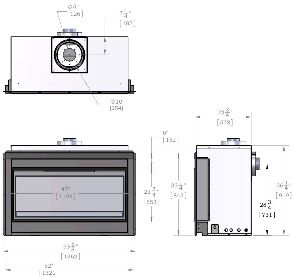
Figure 2. Fireplace dimensions (Tolerance \pm \frac{1}{8}" ).
