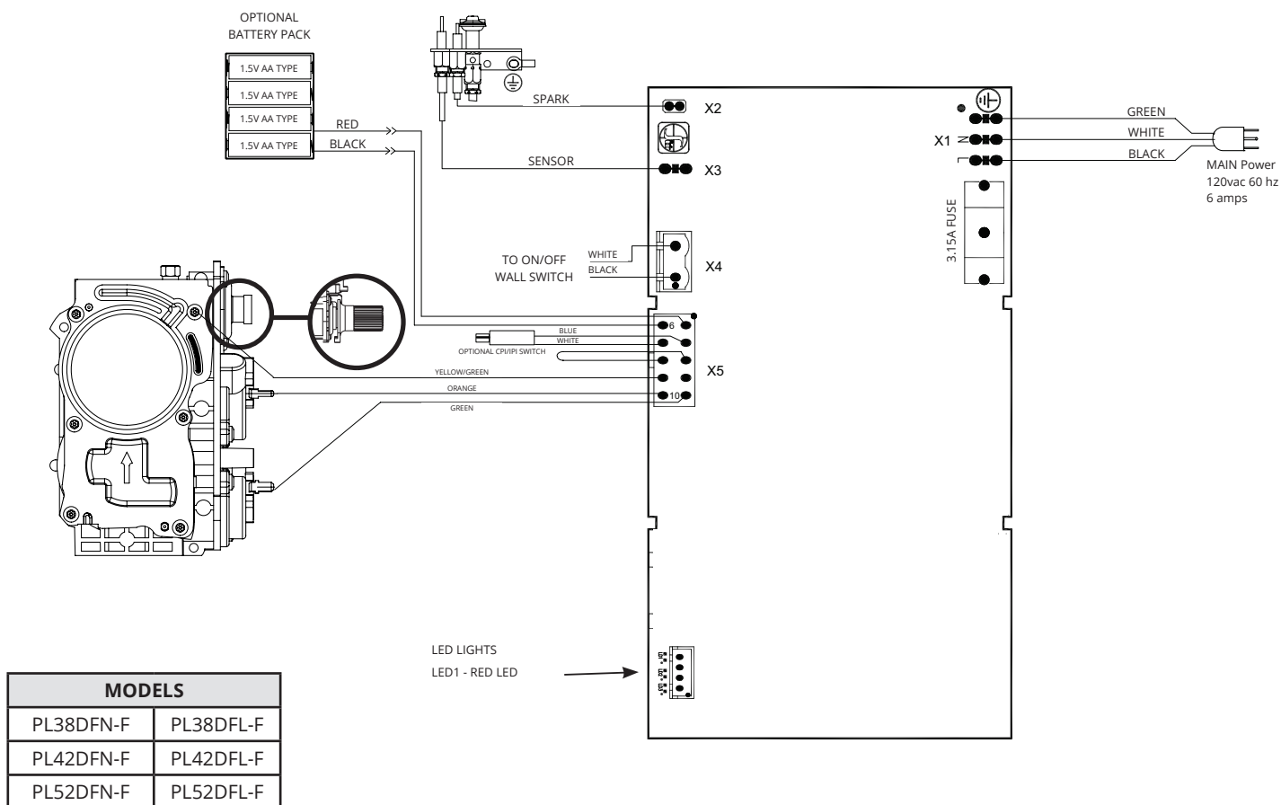
Figure 18. Wiring diagram for PL38DF, PL42DF, PL52DF with SIT Profame BASIC Electronic Ignition
