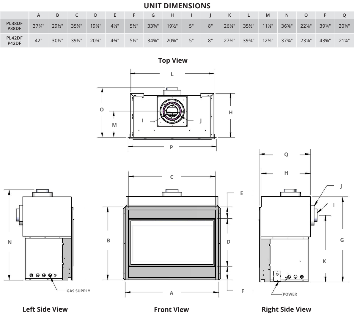
Figure 2. Fireplace dimensions (Tolerance ± 1/8").
