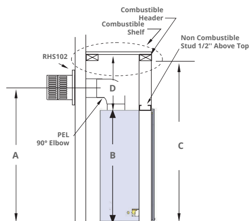
Figure 3.d Combustible Framing for shelves over the fireplace, Top vent.
