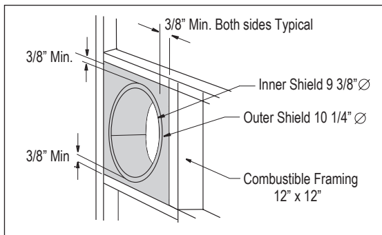
Figure 14. RHS101 Installation. (Install by sliding over vent pipe where it passes through the combustible construction).
