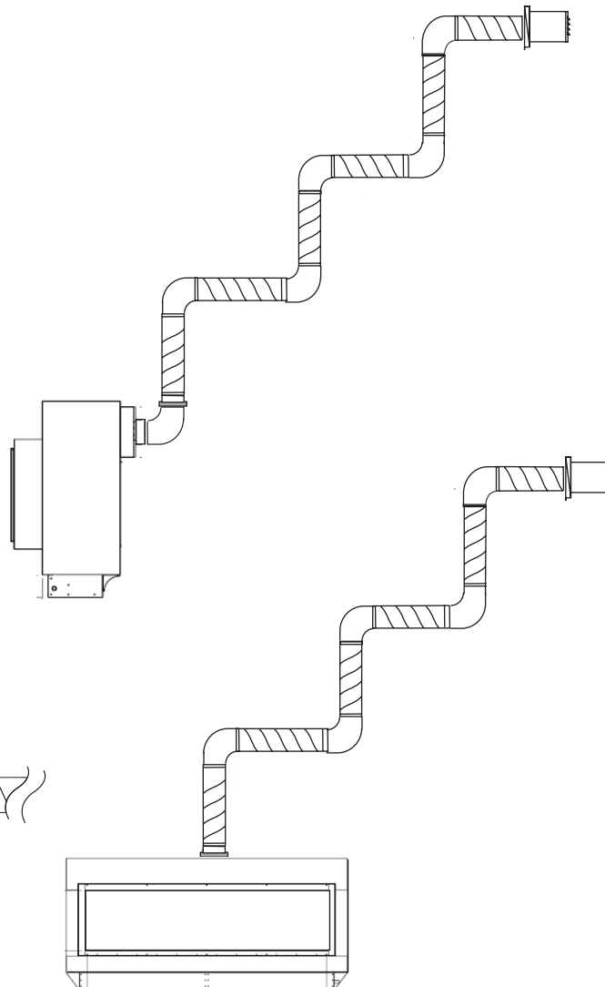
Figure 12b. Multi-Elbow, Top or Rear Vent, Wall mounted power vent.
