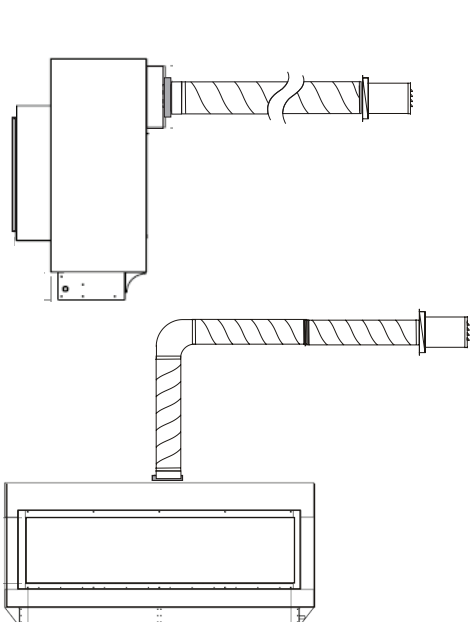
Figure 12. Straight Horizontal, Top or Rear Vent, Wall mounted power vent.
