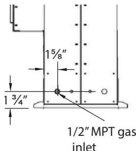
Figure 17. Gas Inlet Supply location.
