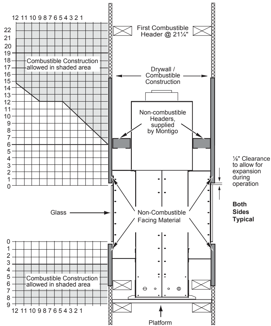
Figure 6 Sec.3 Combustible mantles and facings. (Not to scale)
