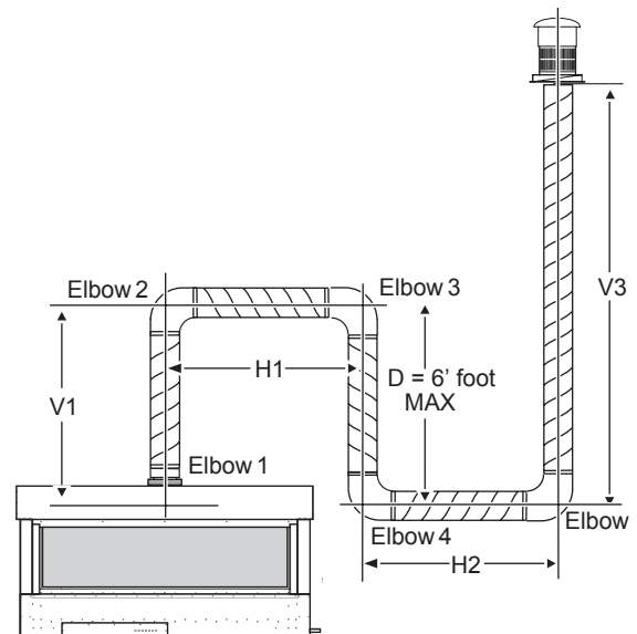
Figure 2 Sec.4 Multi-elbow Venting Installations.
