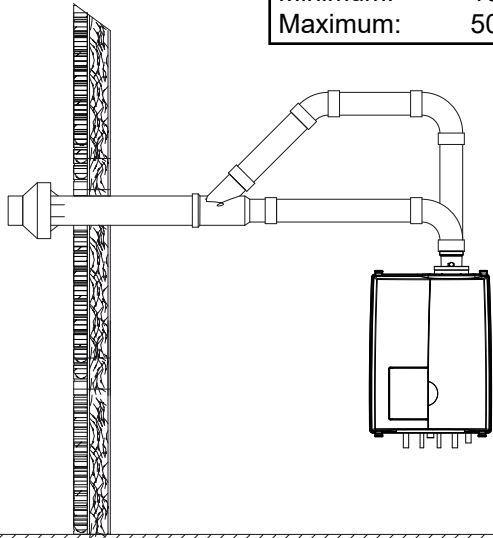
Horizontal with concentric termination figure 12A
