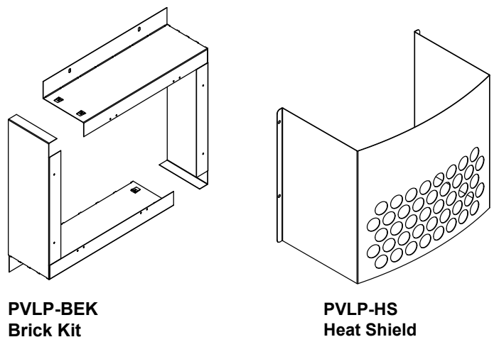
Figure 12.6 PVLP-SLP Vent Components
