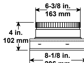
SLP-LPC SLP Low Profile Cap (Approved for use with PVI-SLP-B only)
