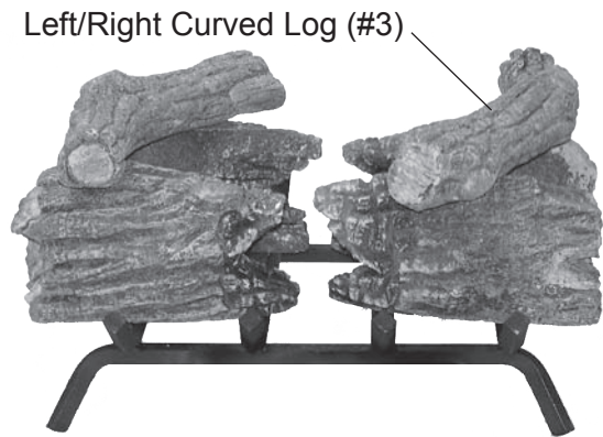
Figure 4 - Placing Left/Right Curved Log (#3) on Bottom Right Logs
