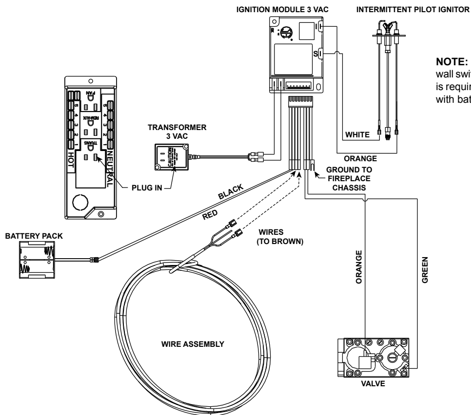
Figure 8.2 Intellifire Pilot Ignition (IPI) Wiring Diagram with Wall Switch or Thermostat (Standard)
