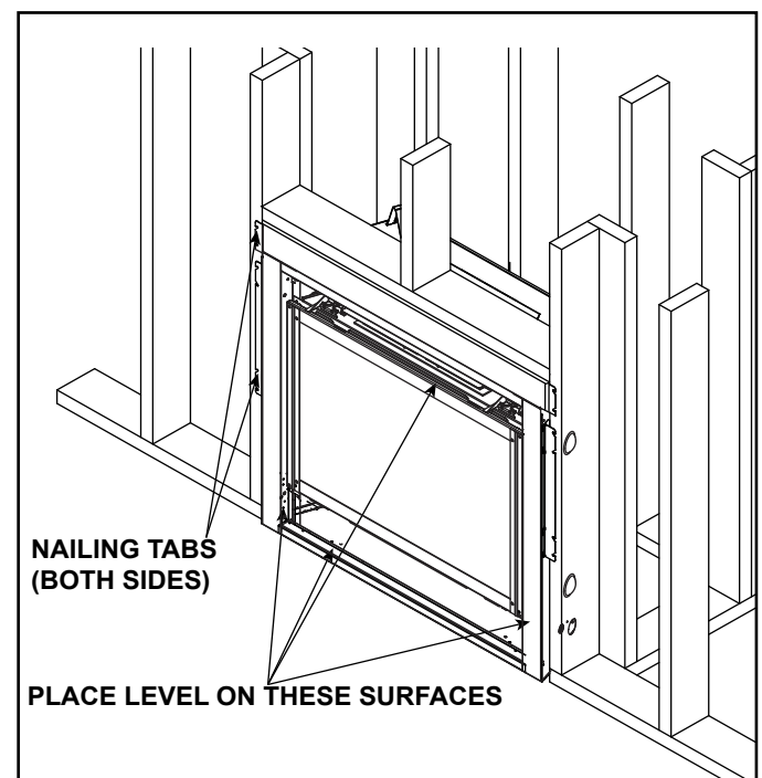
Figure 6.18 Proper Positioning and Securing of an Appliance
