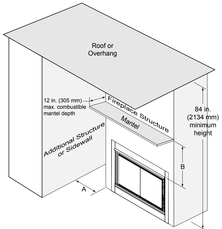
Figure 3.3 Clearances to Mantels or Other Combustibles Above Appliance
