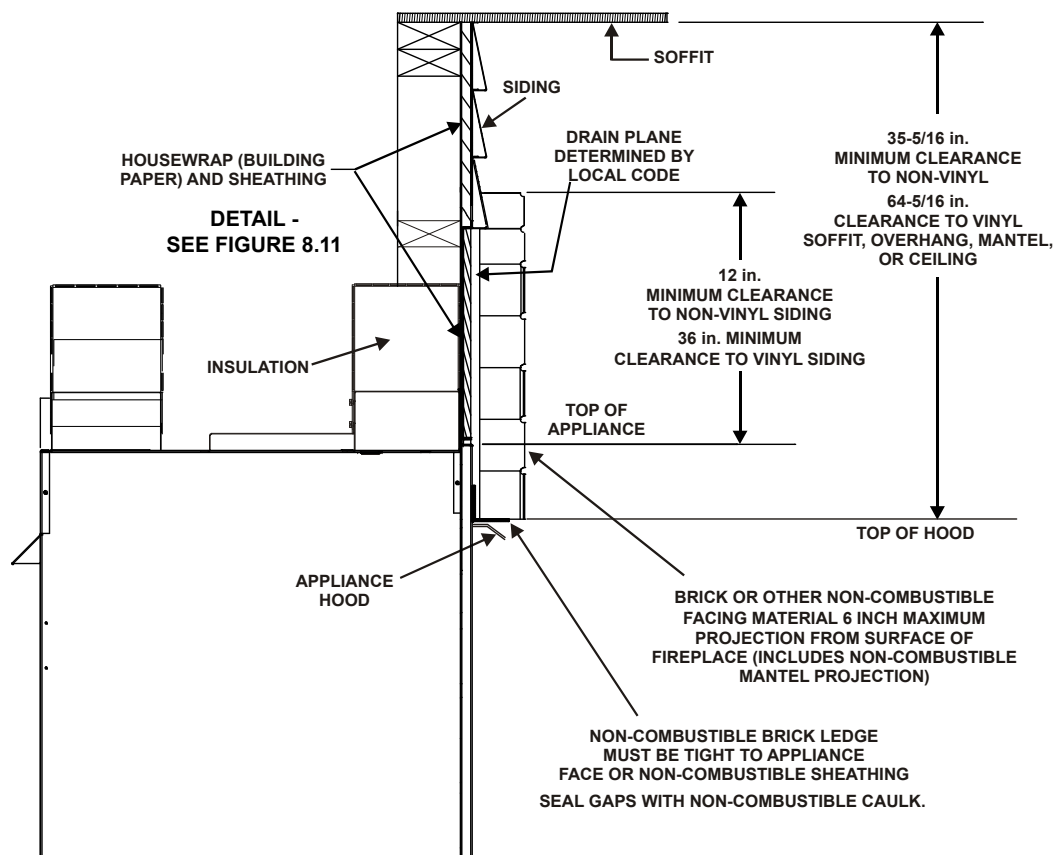
Figure 8.12 Exterior View with Non-combustible Facing Material
