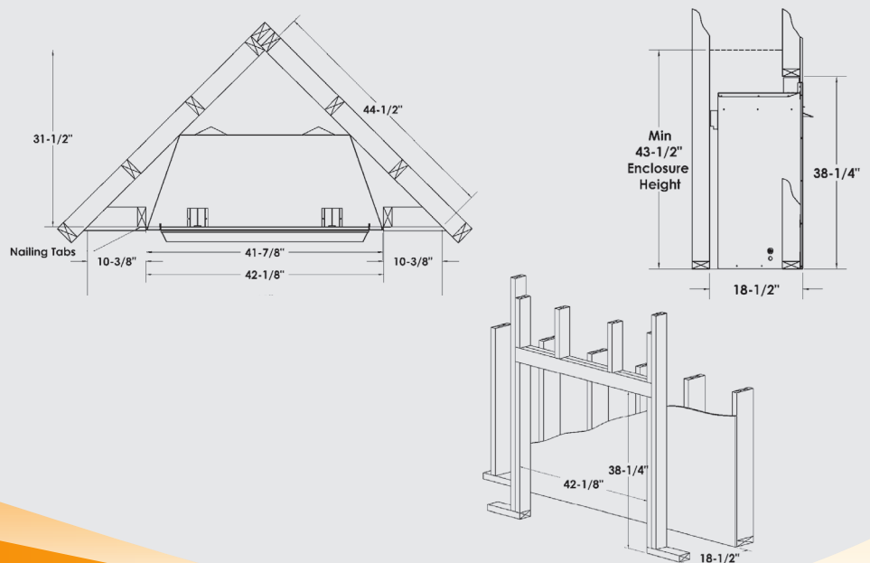
OFP42NS Outdoor Fireplace in Stainless Steel (Natural Gas), LOGF37 Split Oak Log Set, OFP42RLH Herringbone Brick Liner.
