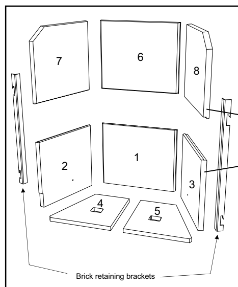
Diagram 1 - Brick Layout
