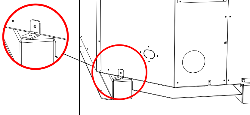
Diagram 3 Anti-Tip Stability Bracket Installation
