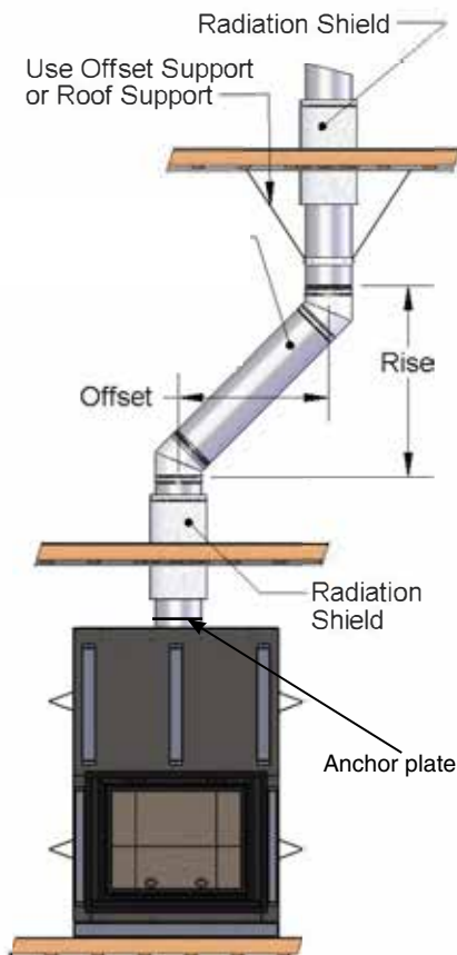
Offset Chimney Installation Example
