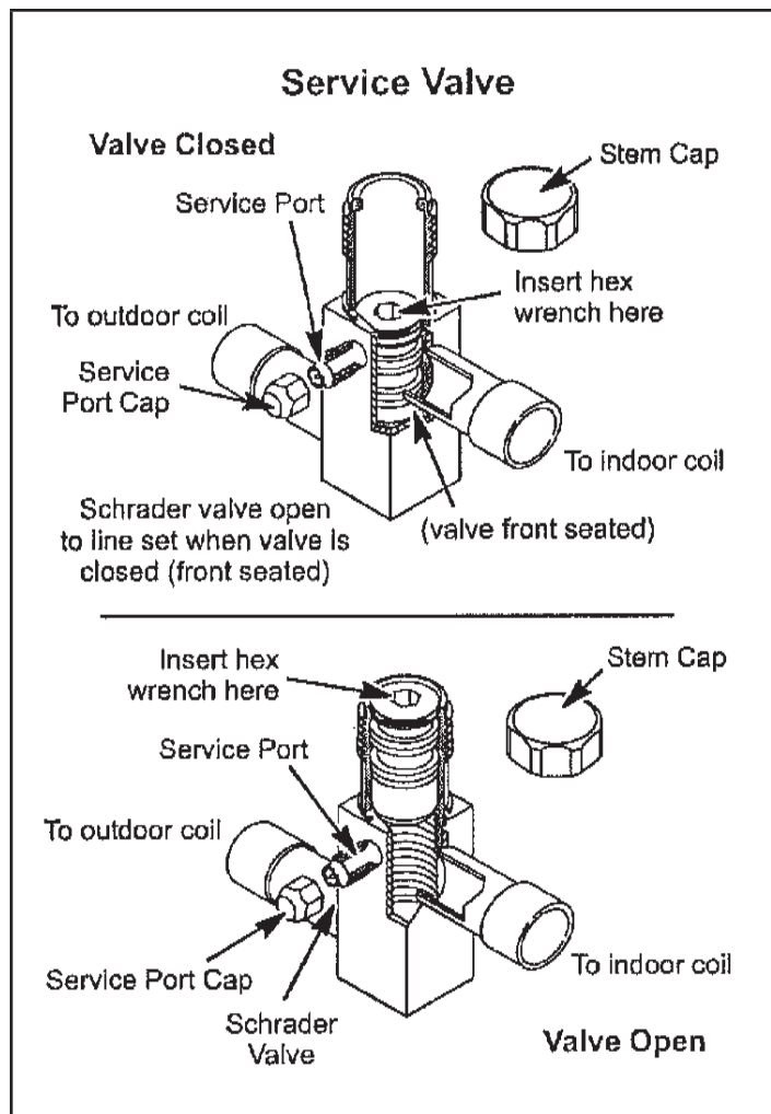
Figure 22. Service Valve
