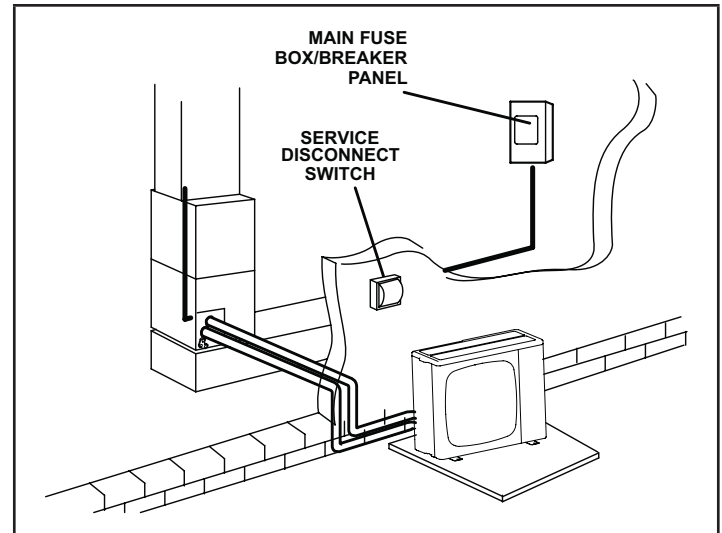
Figure 17. Circuit Installation
