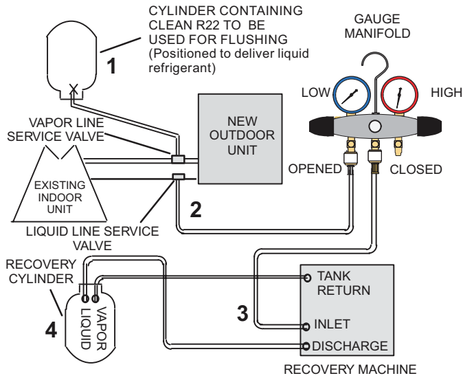
Figure 15. Connecting Gauges
