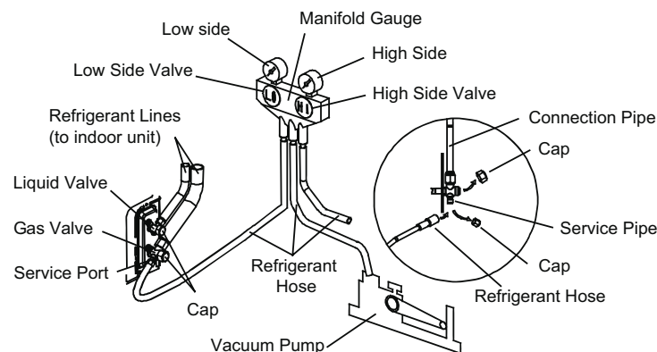
Figure 14. Gauge Connections
